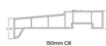
150mm Cill
