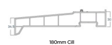
180mm Cill
